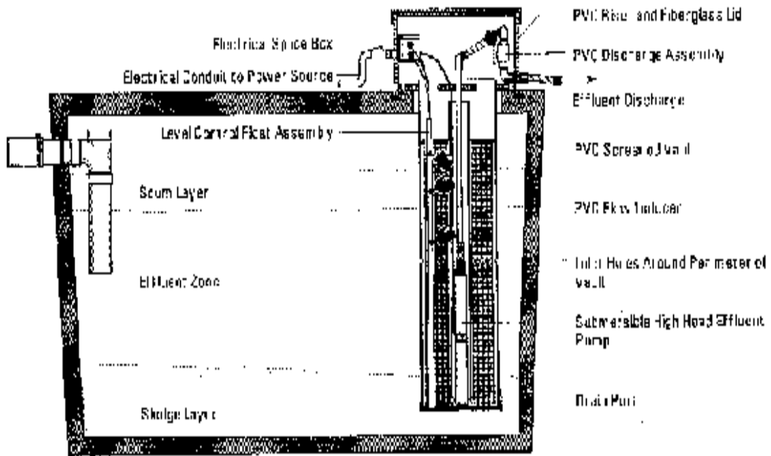
Figure 1 Septic Tank Effluent Pump
