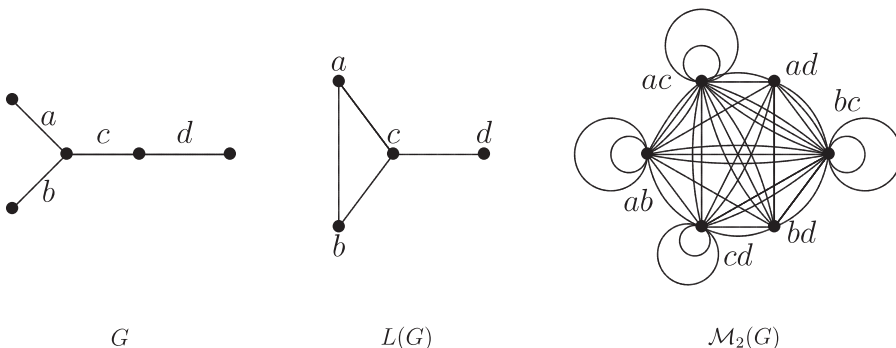
Figure 1. A graph G , its line graph L(G) and super line graph \mathcal{M}_2(G) .
