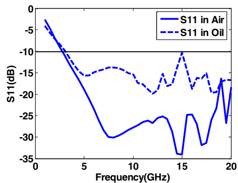
Figure 1: S11 of Modified Fourpoint in Air and Oil
