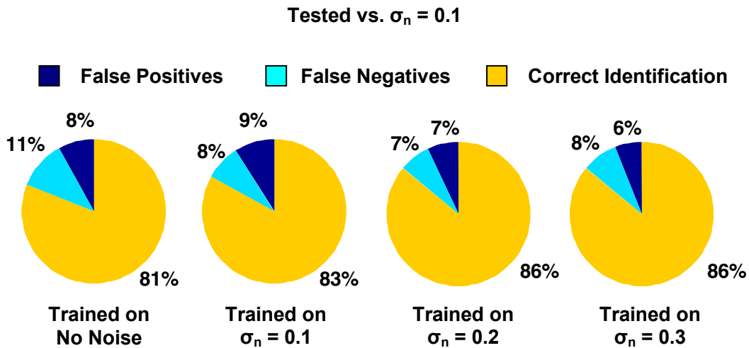
Figure 3: Results for various training networks vs. data with \sigma_n = 0.1
