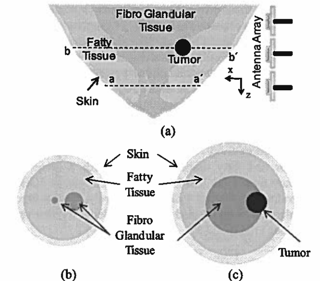
Fig. 2. (a) Breast model developed from MRI scan from [4] with tumor and antenna array, (b) top view of cross-section a-a', and (c) top view of cross-section b-b'.
