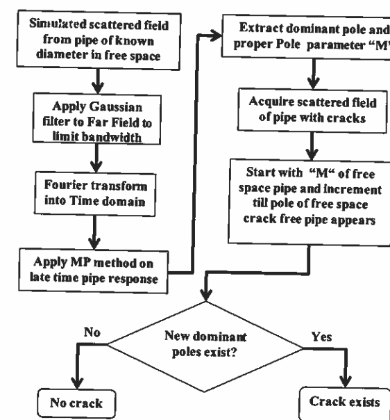
Fig. 17. Pole extraction algorithm.
