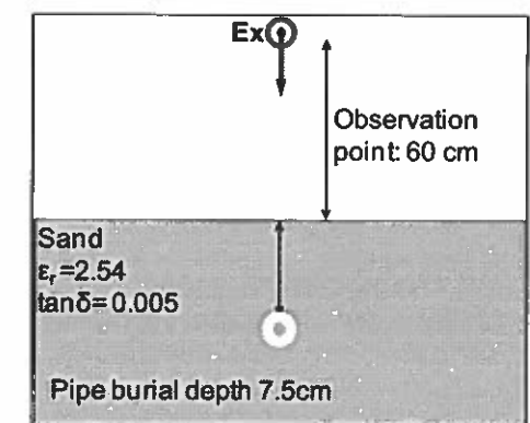
Fig. 13. Configuration of the pipe buried underneath sand.
