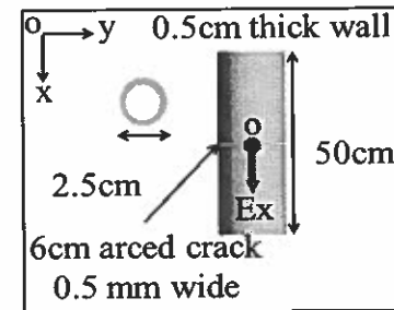
Fig. 1. Pipe configuration and dimensions.
