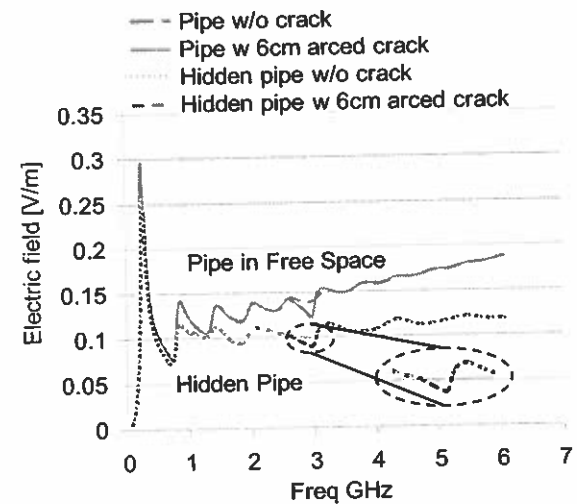
Fig. 9. Comparison of scattered field for pipe in free space vs. pipe hidden behind plywood.
