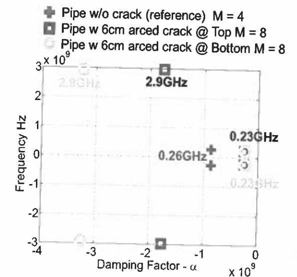
Fig. 5. Pole comparison for reference pipe with no cracks vs. same pipe with 6.0 cm arced crack.
