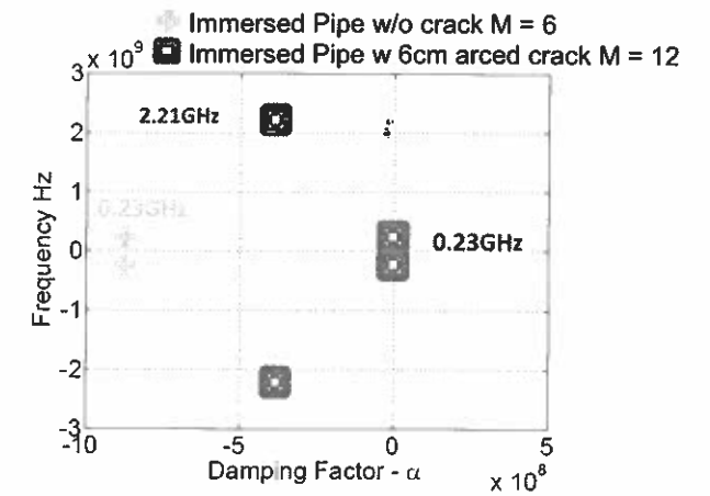
Fig. 12. Pole comparison for immersed pipe cases.
