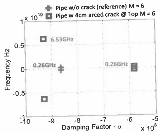
Fig. 7. Pole plot for the reference pipe with and without the 4.0 cm arced crack.
