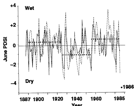
Fig. 2. Actual (dashed line) and reconstructed (solid line) June PDSI for North Carolina from 1887 to 1985. The full 99-year regression model was used for this reconstruction ( r_{\text{adj}}^2 = 0.47 , Table 1). The Palmer index scales drought (-) and wetness (+) anomalies as: 0 to \pm 1 = near normal; \pm 1 to \pm 2 = mild; \pm 2 to \pm 3 = moderate; \pm 3 to \pm 4 = severe; \leq -4 = extreme drought, \geq +4 = extreme wetness. The means for three significantly different June PDSI regimes on the basis of the actual statewide data are indicated by the horizontal dotted lines (1891 to 1924, 1925 to 1955, 1956 to 1984), along with the overall mean (solid line). The North Carolina June PDSI observed in 1986 (circle) was the lowest recorded value in 100 years (3).
