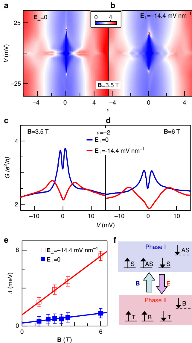
Figure 3 | Transport spectroscopy data from device 1. (a,b) G(V, n) at E_{\perp} = 0 and -14.4 mV nm ^{-1} , respectively. Data are taken at B = 3.5 T. (c) Line traces G(V) at \nu = -2 and B = 3.5 T. Blue and red traces are taken at E_{\perp} = 0 and -14.4 mV nm ^{-1} , respectively. (d) Similar data taken at B = 6 T. (e) Measured LL gap \Delta(B) at \nu = 2 and E_{\perp} = 0 and -14.4 mV nm ^{-1} , respectively. Error bars are estimated from bias resolution and uncertainties in the valley width measurement. (f) Schematics of transitions between phases I and II at \nu = 2 . (T/B, top/bottom layer; S, symmetric state |S\rangle := |T\rangle + |B\rangle ; |AS\rangle : antisymmetric state |T\rangle - |B\rangle ).
