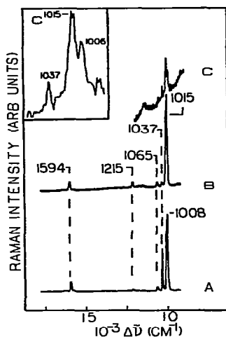
Fig. 1. Surface enhanced Raman (SER) spectra from pyridine adsorbed on electrode surfaces. Curve A is pyridine on an anodized Ag surface E_{\text{appl.}} = -0.6 \text{ V} Laser power, 120 mW at 635 nm. Curve B: as in A but on a Cu surface. Curve C SER spectrum of pyridine on an unanodized Cu electrode. Laser power 120 mW at 645 nm. Vertical scale expansion factors are A = 1X (no expansion), B = 6X, C = 70X and inset C = 180X.
