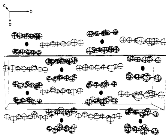
Figure 2. Unit cell of (\text{DMeFe})(\text{TCNQ}) viewed down the c axis. One of the CN groups of \text{TCNQ}^- has been replaced by O showing the \text{DCTC}^- ion. The \text{DMeFe}^+ cation is shaded.
