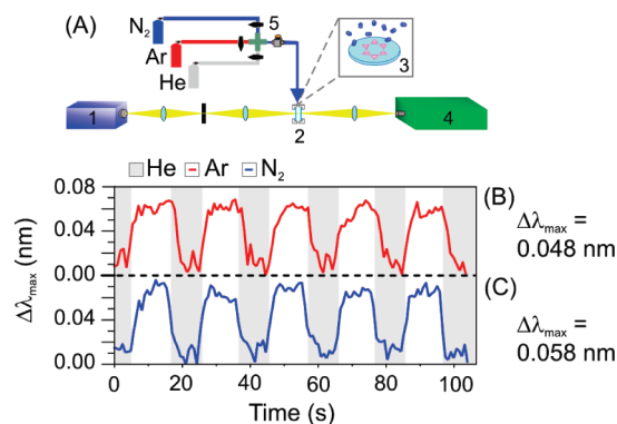
Figure 1. (A) HR-LSPR gas detection apparatus: (1) lamp, (2) flow cell, (3) nanoparticle substrate, (4) HR-LSPR spectrometer, (5) gas-dosing system. (B, C) Plots of LSPR extinction maximum of Ag nanoparticles vs time as the gas was switched between (B) He(g) (shaded areas) and Ar(g) and (C) He(g) and N 2 (g).
