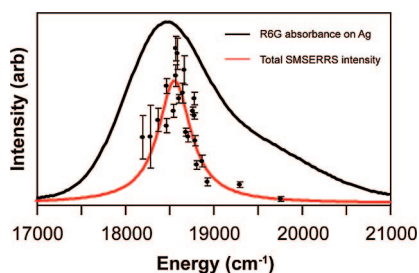
Figure 6. Comparison of the single-molecule surface-enhanced resonance Raman (SM-SERS) of R6G to the ensemble-averaged surface absorbance spectrum on Ag. The single-molecule REP (points) was obtained from the sum of all observed Raman modes and was fit to a Lorentzian function (red solid line) where the error represents one standard deviation from the mean ( E_{max} = 18563 \text{ cm}^{-1} and \text{fwhm} = 449 \text{ cm}^{-1} ). The molecular absorbance of R6G on 200 nm Ag film (black) was fit by a sum of two Gaussians. As expected, the single-molecule data are significantly narrower than the ensemble-averaged analogue ( \sim 1100 \text{ cm}^{-1} ).
