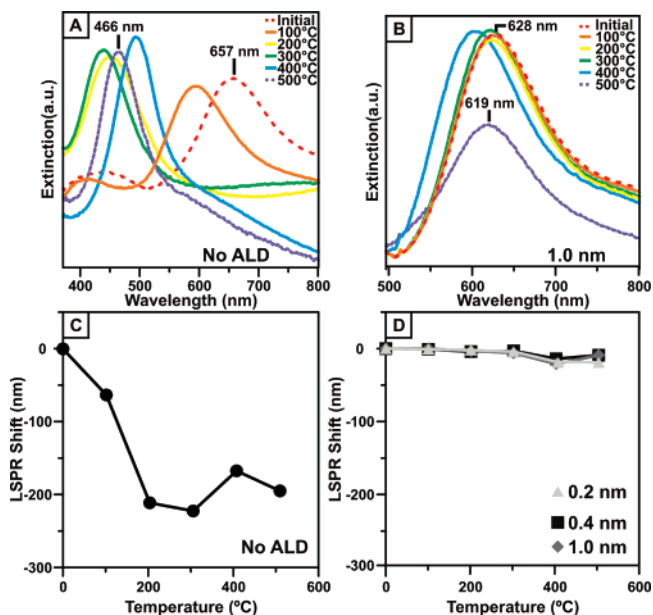
Figure 1. LSPR spectroscopy of bare Ag nanoparticles (A) and Ag nanoparticles coated with 1.0 nm ALD Al 2 O 3 (B) heated at various temperatures. (C) Plot of LSPR shift vs temperature of bare Ag nanoparticles heated at various temperatures. (D) Plot of LSPR shift vs temperature of Ag nanoparticles coated with 0.2 nm (▲), 0.4 nm (■), and 1.0 nm (◆) ALD Al 2 O 3 heated at various temperatures. All samples were heated at each temperature for 1 h under 1 Torr N 2 .
