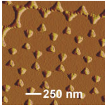
Figure 1. Tapping mode AFM image of the Ag nanoparticle LSPR nanosensor. After solvent annealing, the resulting nanoparticles have in plane widths of \sim 100 nm and out-of-plane heights of 51 nm. Defects are present in sensing probe volume but do not contribute to the optical sensing events.
