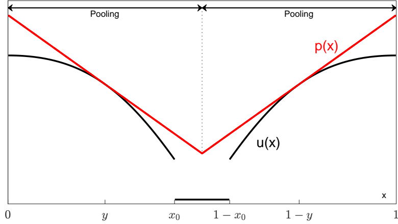
Figure 9: Portfolio recommendation: concave case
