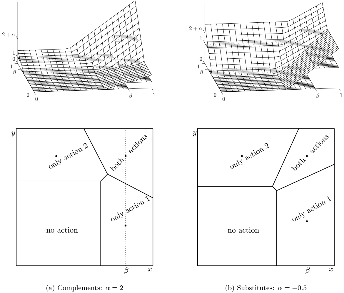
Figure 11: Solution of the multidimensional persuasion problem for complements (left panels) and substitutes (right panels). The top row shows u (fine mesh, in background) and p (coarse mesh, in foreground). The bottom row shows the pooling regions, which actions they induce, and how the centers of mass of the regions that induce some action lie on the threshold \beta . The pooling regions correspond to the affine regions of p . Other parameters: \beta = 0.8 , F = bivariate uniform.
