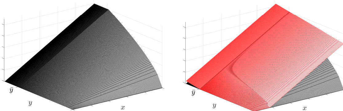
Figure 12: The objective function v(x, y) (left panel) and the objective function with the supporting prices p(x, y) (right panel)
