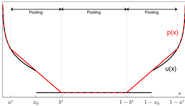
Figure 10: Portfolio recommendation: convex case
