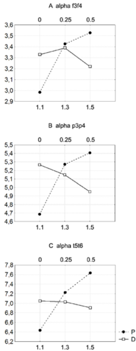
Fig. 2. Plot of main results and interactions. Combined means in \mu\text{V} on the y-axis, for the three levels of randomness (P) and the three fractal dimensions (D) on the x-axis. Dotted line represents P, continuous line represents D. Panel A: alpha F3F4; Panel B: alpha P3P4; Panel C: alpha T5T6.
