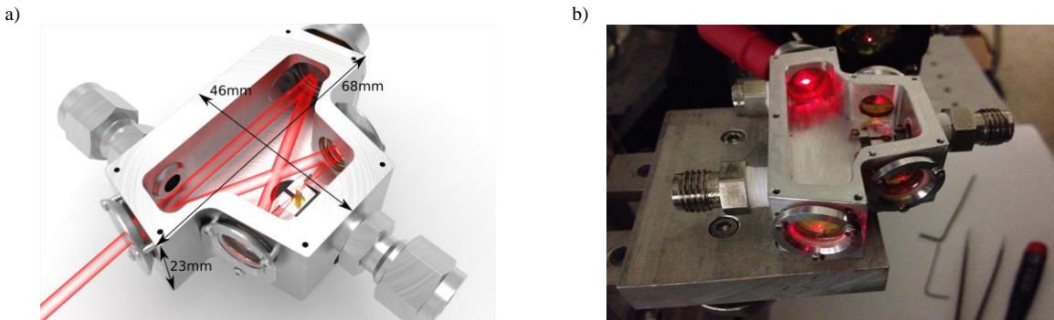
Fig. 2. (a) Compact intra cavity QEPAS stainless ADM module, resulting in a ~ 5000 fold power enhancement. (b) A red diode laser beam was used for alignment of the mid-IR ICL and QCL pump beams.
