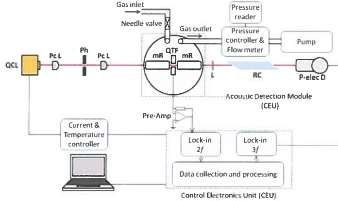
Figure 1: Schematic configuration of a high power 4.61 \mu\text{m} CW RT TEC DFB-QCL based QEPAS system for ppbv detection of CO and N 2 O. Pc L – plano-convex lens, Ph – pinhole, QTF – quartz tuning fork, mR – acoustic micro-resonator, RC – reference cell.
