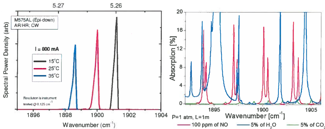
Figure 7: (a) Emission spectra of 1900 cm -1 TEC CW DFB QCL and (b) HITRAN simulated spectra of NO, H 2 O, and CO 2 .
