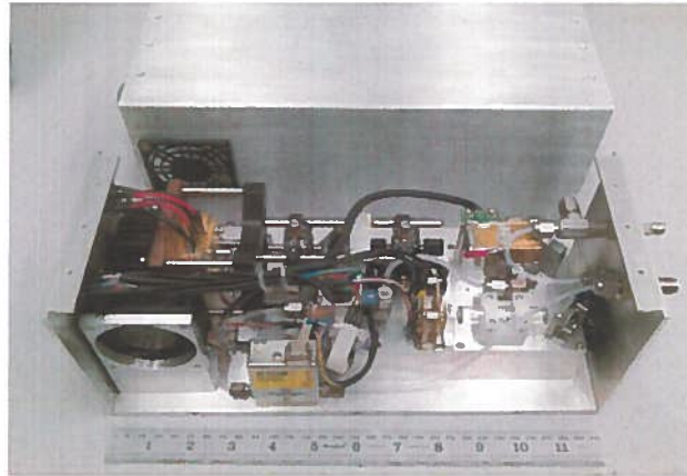
Figure 8: Compact Prototype NO Sensor.
