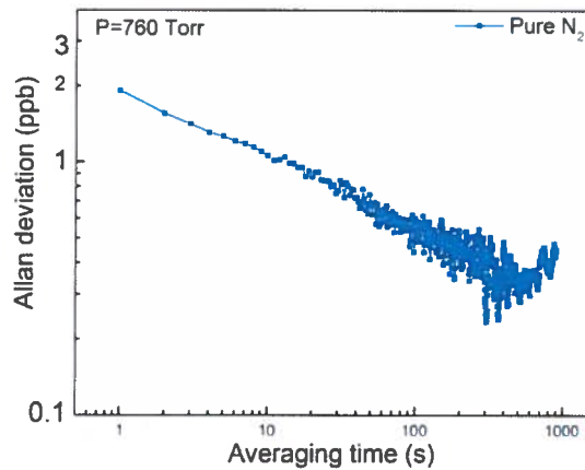
Figure 5: Allan deviation plot for time series measurements of pure N_2 for the QEPAS based CO sensor system.
