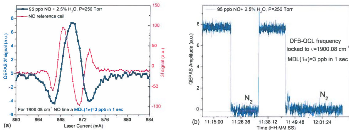
Figure 9: 2f QEPAS signal amplitude when QCL frequency is tuned across (a) and locked (b) to the NO doublet absorption line at 1900.08 \text{ cm}^{-1} .
