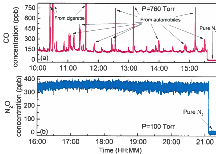
Figure 6: Continuous monitoring of atmospheric CO and N_2O concentration levels from an air sampled on Rice University campus, Houston, TX, USA (Latitude and longitude are: 29^\circ 43' N/95^\circ 23' W ). (a): CO concentration measurements; (b): N_2O concentration measurements.
