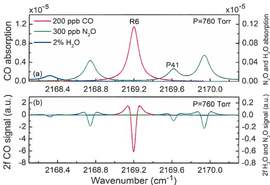
Figure 3: HITRAN based simulation spectra of CO and \text{N}_2\text{O} at a temperature of 296 K, a standard atmospheric pressure, an optical path length of 1 cm for 200 ppbv CO, 2% \text{H}_2\text{O} and 300 ppbv \text{N}_2\text{O} , respectively. (a): absorption spectra; (b): 2^{\text{nd}} harmonic absorption spectra.
