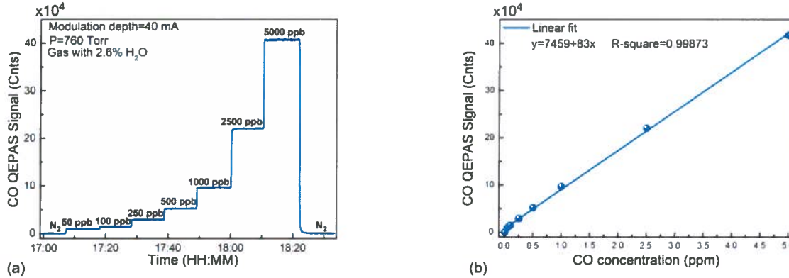
Figure 4(a): QEPAS signal amplitude recorded in the line locking mode as the CO concentration is varied at atmospheric pressure and a modulation depth of 40 mA. (b): QEPAS signals amplitude averaged from Fig. 4(a) as a function of CO concentration. 1cnt = 6.67 \times 10^{-16} A.
