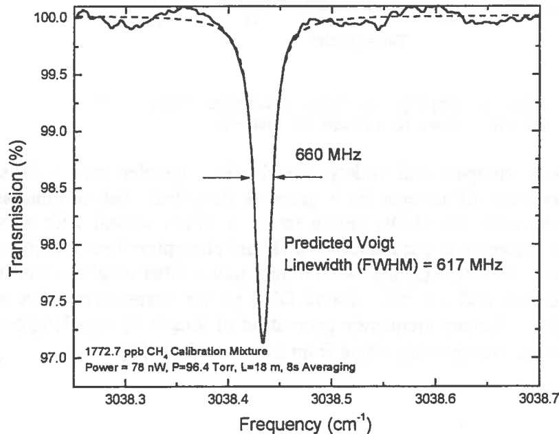
Fig. 4: Methane absorption line at 3038.52 cm -1 acquired from a calibrated gas mixture
