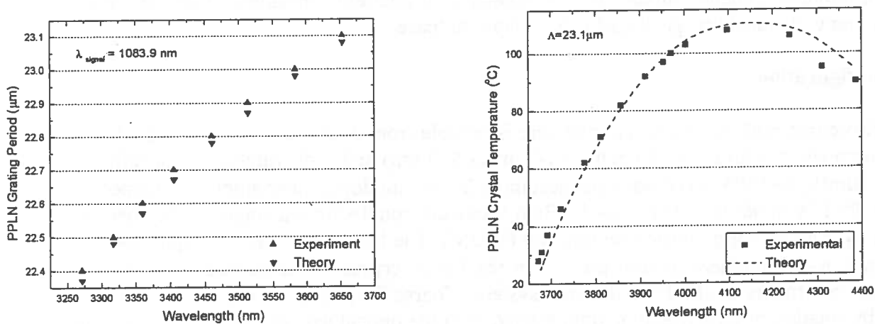
Fig. 3: Two quasi-phase matching approaches by changing the nominal grating period (a) or temperature tuning at a fixed nominal grating period (b)
