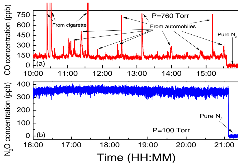
Fig. 6: Continuous monitoring of atmospheric CO and N_2O concentration levels from an air sampled on Rice University campus, Houston, TX, USA (Latitude and longitude are: 29^\circ 43' N/95^\circ 23' W ). (a): CO concentration measurements; (b): N_2O concentration measurements.
