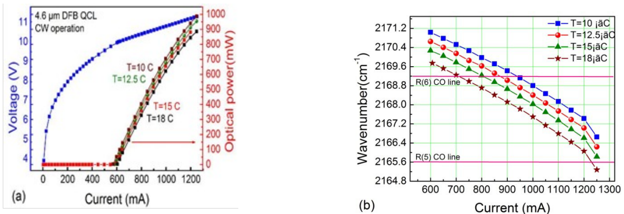
Figure 2: 2(a) LIV curve of a 4.61 \mu\text{m} RT, CW, DFB-QCL from Center for Quantum Devices, Northwestern University; (b) DFB-QCL current tuning at different operating temperatures.
