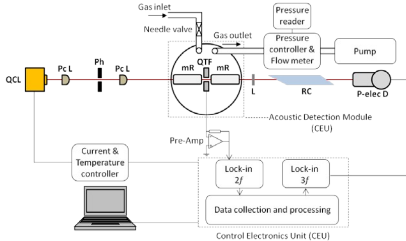
Fig. 1 Schematic configuration of a high power 4.61 \mu\text{m} CW RT TEC DFB-QCL based QEPAS system for ppb detection of CO and \text{N}_2\text{O} . PcL – plano-convex lens, Ph – pinhole, QTF – quartz tuning fork, mR – acoustic micro-resonator, RC – reference cell.
