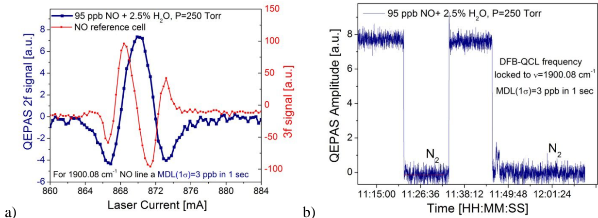
Fig 9. 2f QEPAS signal amplitude when QCL frequency is tuned across (a) and locked (b) to the NO doublet absorption line at 1900.08 cm -1 .
