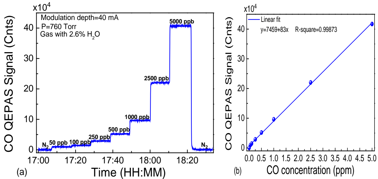
Fig. 4(a): QEPAS signal amplitude recorded in the line locking mode as the CO concentration is varied at atmospheric pressure and a modulation depth of 40 mA. (b): QEPAS signals amplitude averaged from Fig. 4(a) as a function of CO concentration. 1cnt = 6.67 \times 10^{-16} A.
