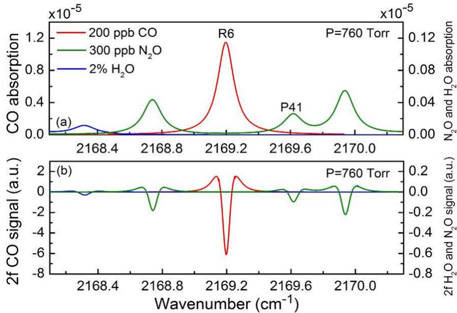
Fig. 3 HITRAN based simulation spectra of CO and N 2 O at a temperature of 296 K, a standard atmospheric pressure, an optical path length of 1 cm for 200 ppb CO, 2% H 2 O and 300 ppb N 2 O, respectively. (a): absorption spectra; (b): 2nd harmonic absorption spectra.
