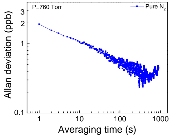
Fig. 5: Allan deviation plot for time series measurements of pure N_2 for the QEPAS based CO sensor system.
