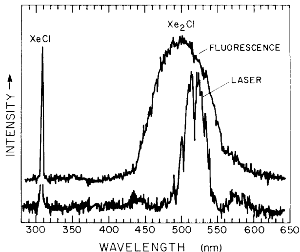
FIG. 3. Fluorescence and laser spectrum of Xe 2 Cl and XeCl ( B \rightarrow X ) of an Ar/Xe/CCl 4 mixture of 6.5 atm, 200 Torr, and 1 Torr, respectively. All intensities are shown in arbitrary units, not corrected for the spectral response of the OMA Model 1205D/01 vidicon detector.
