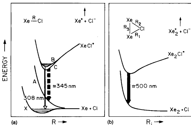
FIG. 2. Simplified potential-energy diagram of the diatomic excimer XeCl and triatomic excimer Xe 2 Cl.
