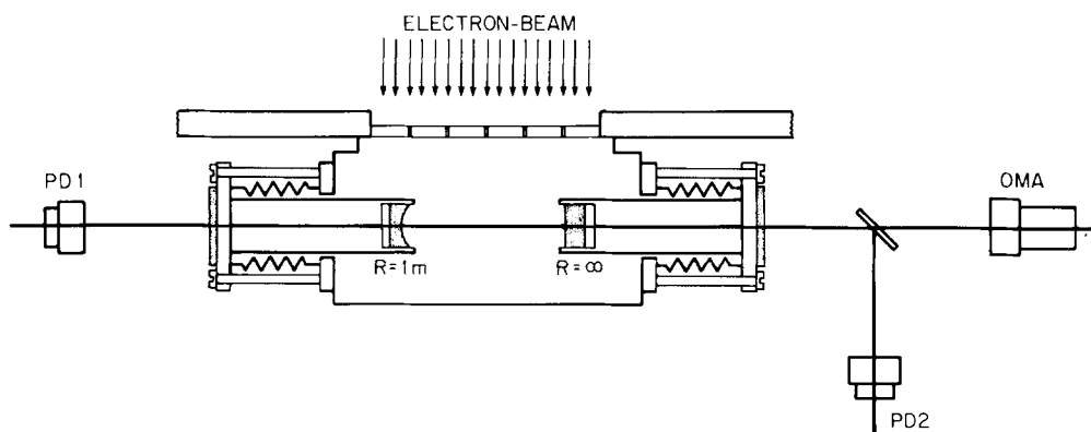
FIG. 1. Schematic of electron-beam-pumped laser cell and associated diagnostic instrumentation.
