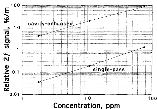
Fig. 8. Measured relative 2f signal amplitude per unit cell length P_{2f}/(P_{0f}L) in the case of single-pass and cavity-enhanced detection, versus concentration of methane in air at 13.3 kPa (100 torr). The enhancement factor (max. 116) is in good agreement with the measured cavity finesse
