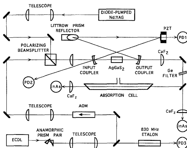
Fig. 1. Experimental setup for spectroscopic detection of methane near 3.2 \mu\text{m} in air. The AgGaS 2 crystal was placed into a bow-tie build-up cavity which was locked to resonance at 1064 nm. The 1064 nm light was supplied by a diode-pumped Nd:YAG laser. The tunable 800 nm light was supplied by either a grating tuned extended-cavity diode laser or a solitary laser diode. The IR power was stabilized by adjusting the diode laser power with an AOM
