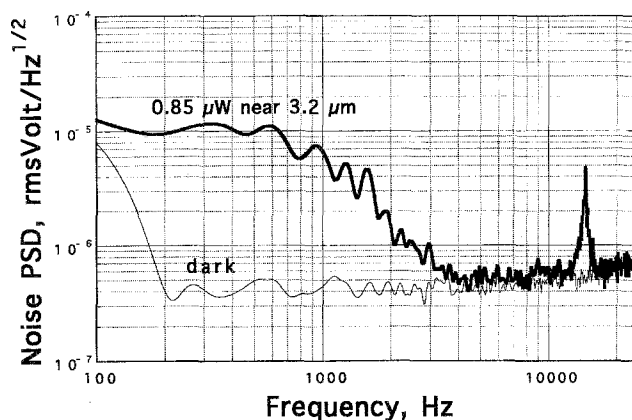
Fig. 4. The power spectral density of the noise from the InSb photo-detector/preamplifier measured with a fast Fourier transform analyzer. The upper curve was taken when the detector was exposed to 0.85 \mu\text{W} of IR DFG radiation near 3.2 \mu\text{m} . Note that the buildup cavity locking noise dominates at frequencies below 3 kHz. The detector/preamplifier responsivity at 3.2 \mu\text{m} was 1.2 \times 10^5 \text{ VW}^{-1}
