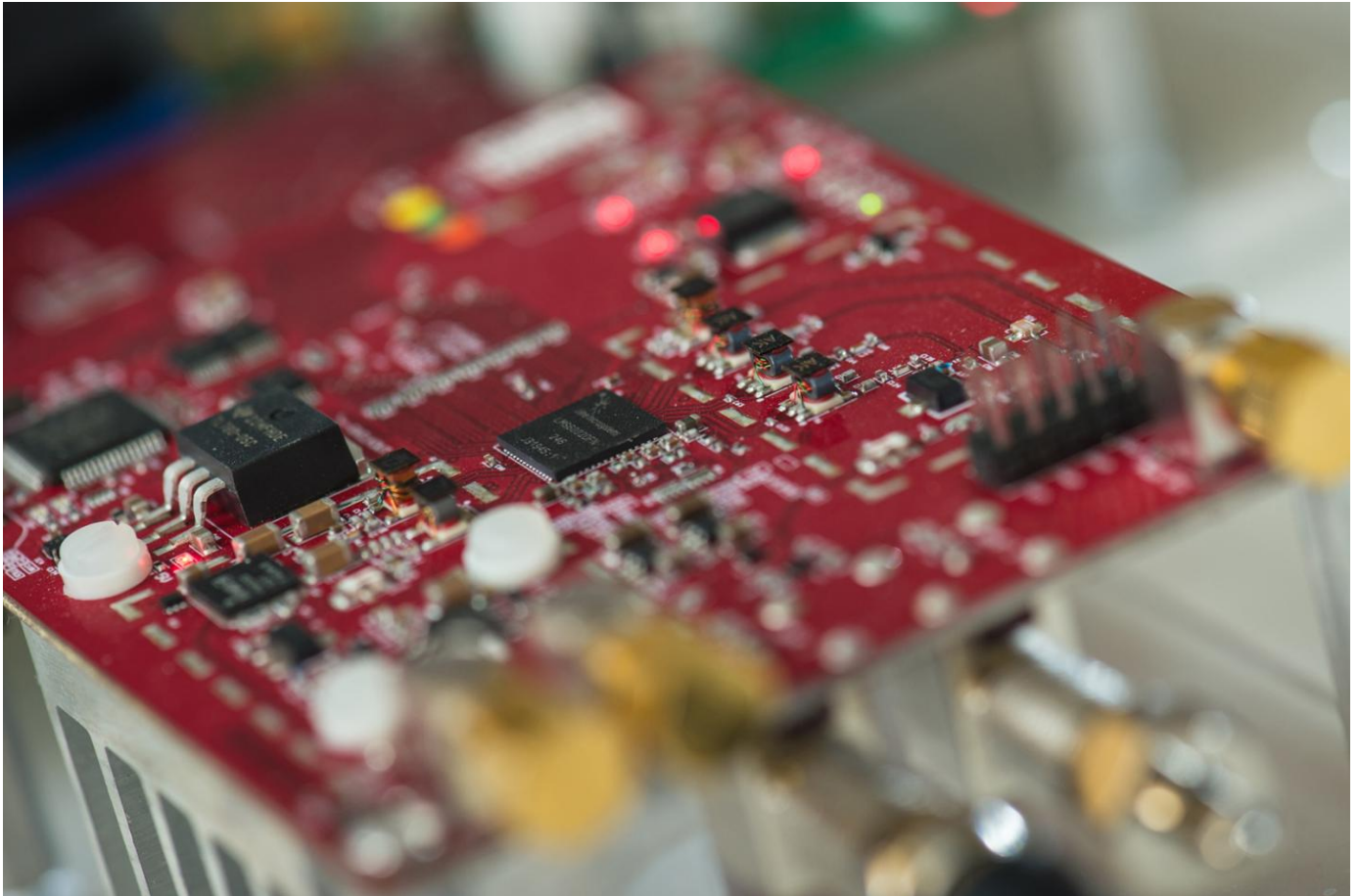
Rice researchers used WARP, the wireless open-access research platform, to build the first system that allows wireless data transmissions over UHF channels during active TV broadcasts. Credit: Jeff Fitlow/Rice University
