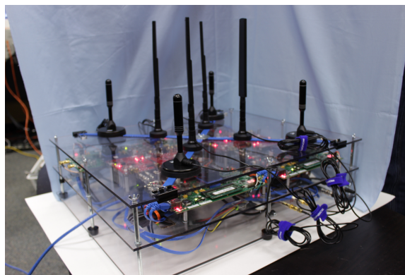
Figure 1: UHF MU-MIMO platform with 4x UHF WURC and 4x 2.4 GHz radios
