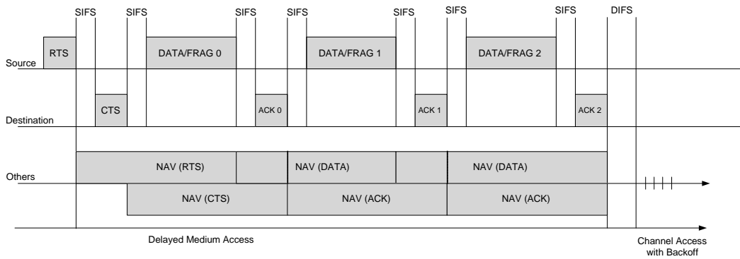
Figure 3: Illustration of fragmentation in IEEE 802.11
