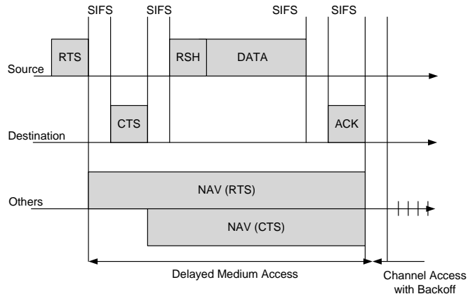
Figure 2: IEEE 802.11 with RBAR enhancement
