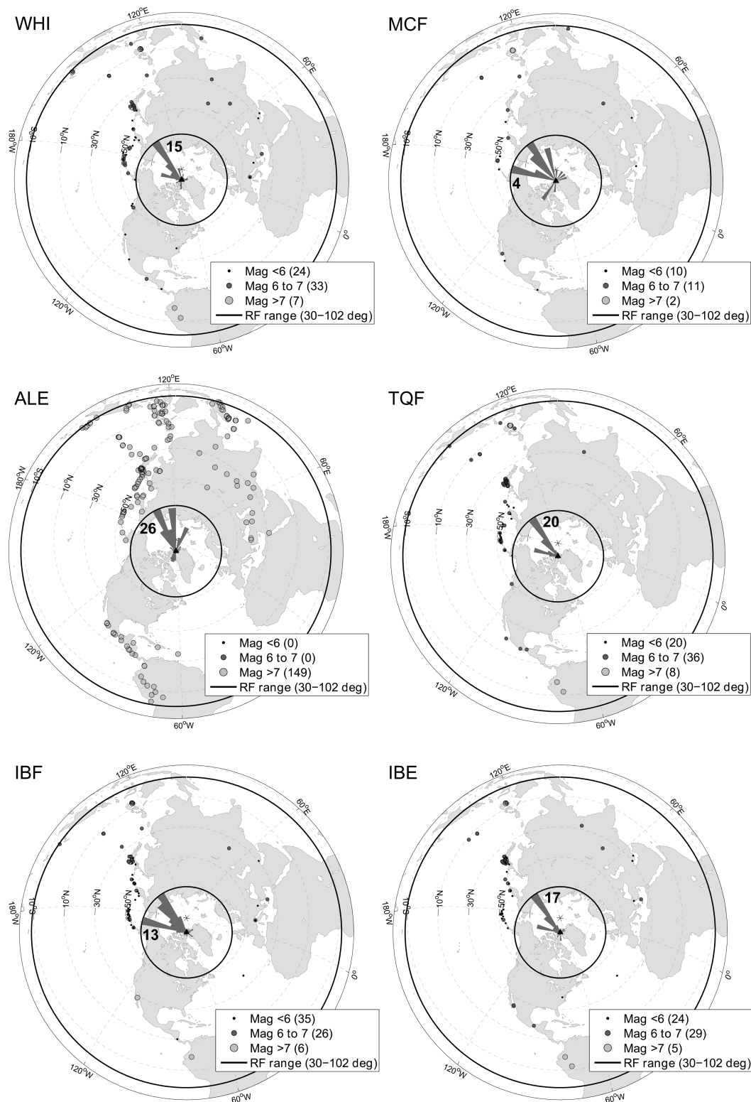
Figure 4. Epicentral plots showing the earthquake locations of all events used for the receiver function processing. The earthquakes are grouped with regard to magnitude (Mag < 6, 6 < Mag < 7, Mag > 7). A histogram of the backazimuth (BAZ) of the events to the station is shown in the centre. The centre indicates zero events, the number inside the inner black circle indicates the maximum number with a linear scale along the radius.
