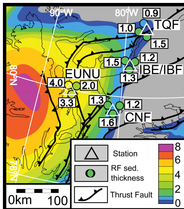
Figure 9. Estimates of the uppermost, low velocity sedimentary layer (Sverdrup Basin) from receiver functions (dots, numerical values in the white boxes in kilometres), defined by the lower boundary of the uppermost steep velocity gradient, compared with sedimentary thickness maps of the Sverdrup Basin (Embry 1990; Oakey & Stephenson 2008).
