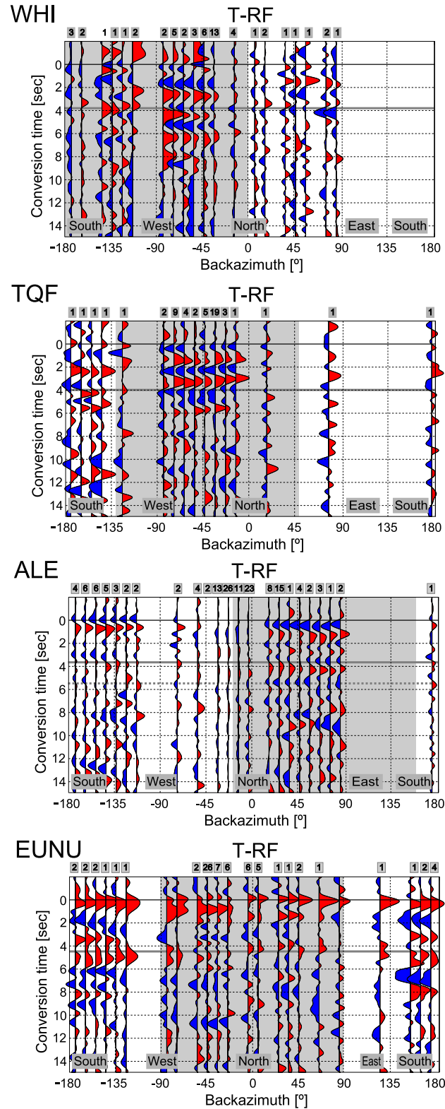
Figure A4. Backazimuth plots for stations WHI, TQF, ALE and EUNU with ‘low frequency’ ( a = 2.5 ) T-RFs (left side). The grey shaded numbers above the single traced indicate the number of stacked RFs for the respective backazimuth range. The grey shaded areas indicate the interpreted backazimuth ranges with of the same RF phases (negative or positive) and the boundary, accordingly, the symmetry axis of the underlying structure.
