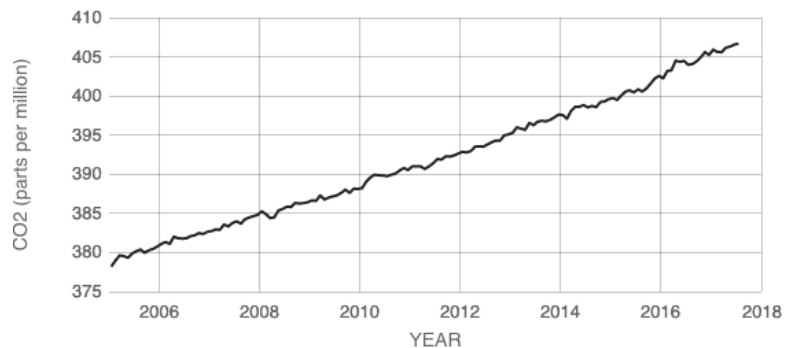
Figure 9: Graph of concentration of carbon dioxide (CO 2 ) in the atmosphere. Image credit: climate.nasa.gov 11
