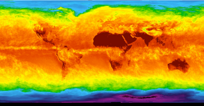
Figure 6. Temperatures on Earth as recorded by an infrared sensor on NASA's Aqua satellite. Credit: AIRS Science Team, NASA/JPL. 7
